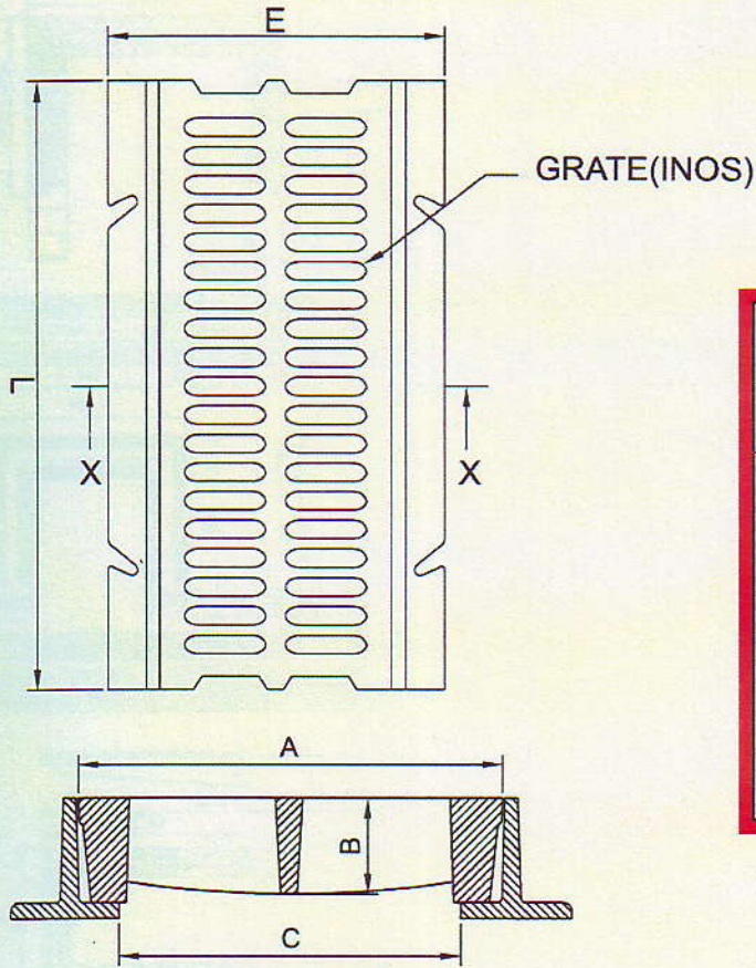
SECTION - "X - X" (ENLARGE VIEW)
